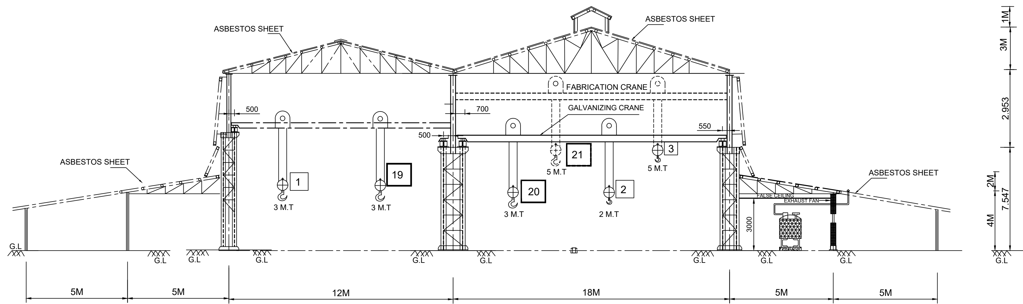
SECTION - X-X (TOWER PLANT)
